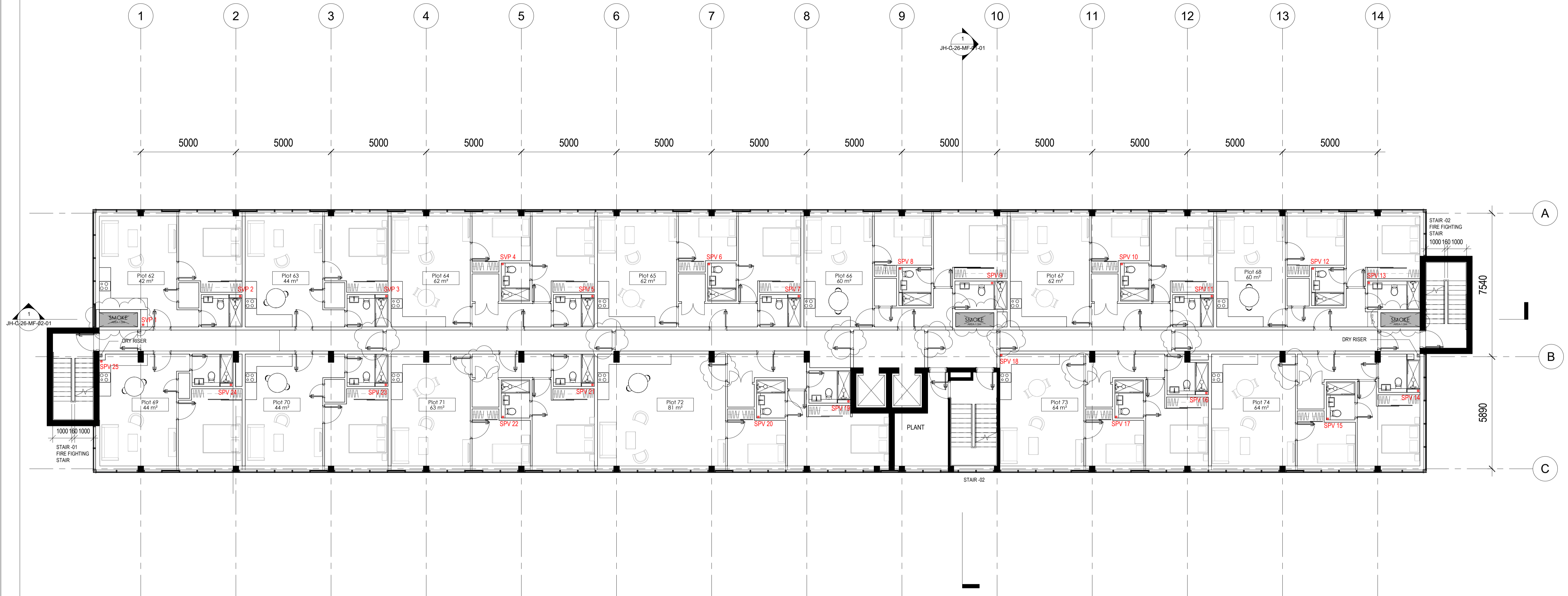
1 FOURTH FLOOR 1 : 100
