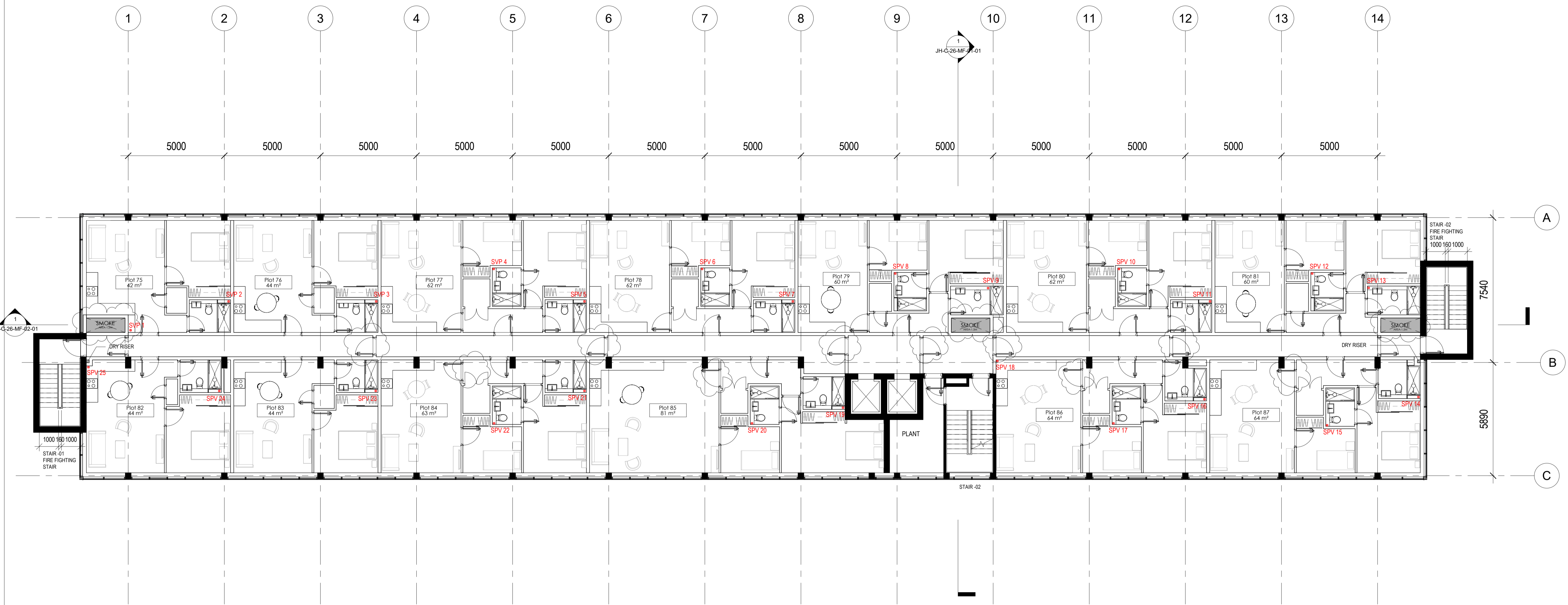
1 FIFTH FLOOR 1 : 100
